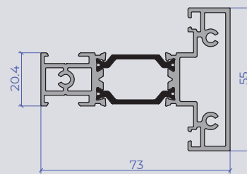
Sash transom
