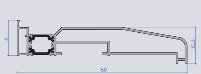
150 mm drainage subcill
