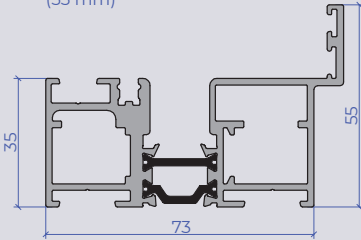
Standard cill outer frame (55 mm)
