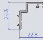
Adjustable jamb rebate
