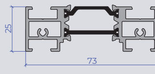
Sliding post/mullion/extension
