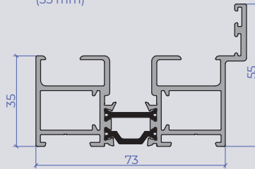
Head/jamb outer frame (55 mm)
