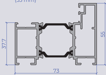
Slim sash (55 mm)
